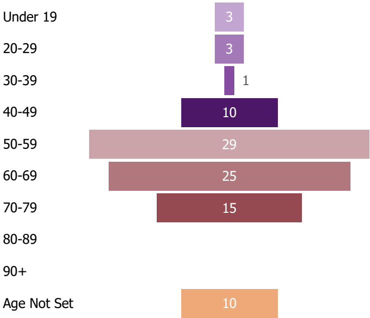
Age Profile: Primary Members
